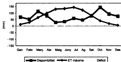
Solana1200 esc = 30 CR = 50
