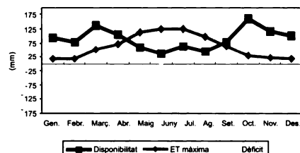
Obaga1200 esc = 30 CR = 75
